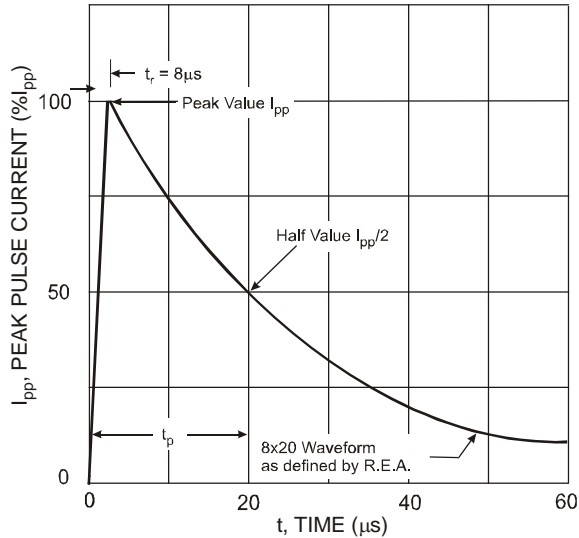
Fig. 1 Pulse Waveform
